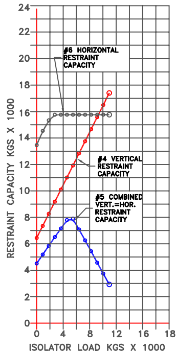
FIGURE 3 CONCRETE ATTACHMENT
